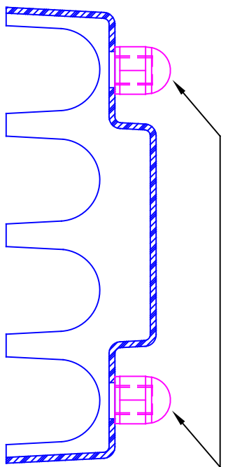
P/N 4001-002 (2 REQ'D.)
